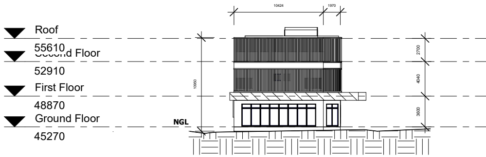
NORTH ELEVATION
