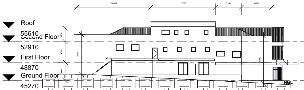
EAST ELEVATION
